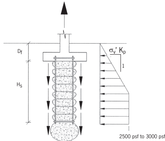
Figure 4. Individual Geopier Pullout Resistance
