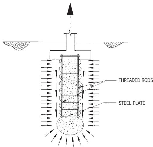
Figure 2. Geopier Uplift Element
