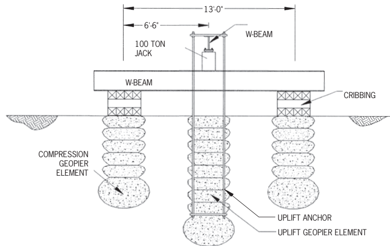
Figure 6. Typical Uplift Load Test Setup
